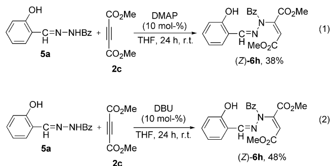
Scheme 4. Reaction of hydrazones 5a (1.0 equiv.) with 2c (3.0 equiv.) in the presence of base catalysts (10 mol-%) at room temperature in THF (2.0 mL).
