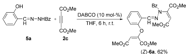
Scheme 2. Reaction of hydrazone 5a (1.0 equiv.) with 2c (2.5 equiv.) in the presence of DABCO (10 mol-%) at room temperature in THF (2.0 mL).
