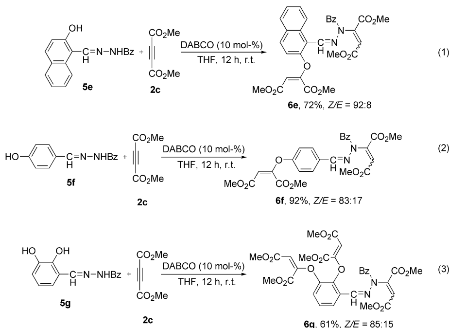
Scheme 3. Reaction of hydrazones 5e , 5f and 5g (1.0 equiv.) with 2c (3.0 equiv.) in the presence of DABCO (10 mol-%) at room temperature in THF (2.0 mL).
