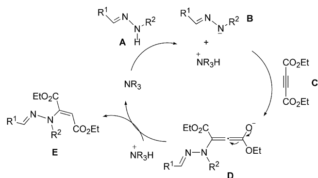
Scheme 5. A plausible reaction mechanism.
